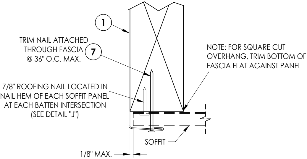
DETAIL "A" Fascia
