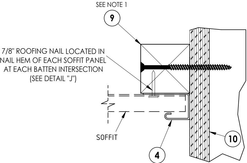
DETAIL "B" J-Channel
