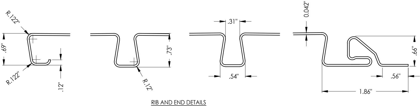
RIB AND END DETAILS
